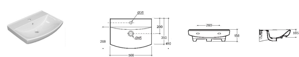
SEMI-RECESSED WASH-BASIN CLAREMONT 50
