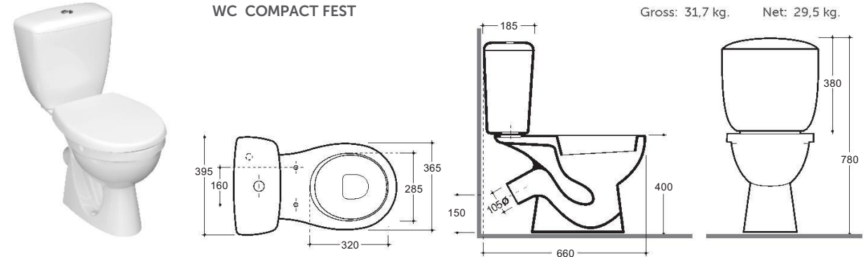
WC COMPACT FEST
