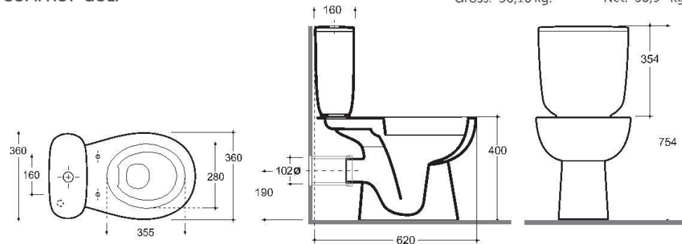
WC COMPACT GOLF
