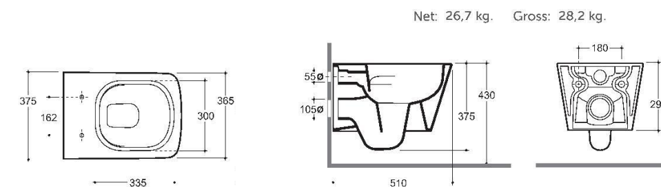
WALL-HUNG WC TOBAGO R
