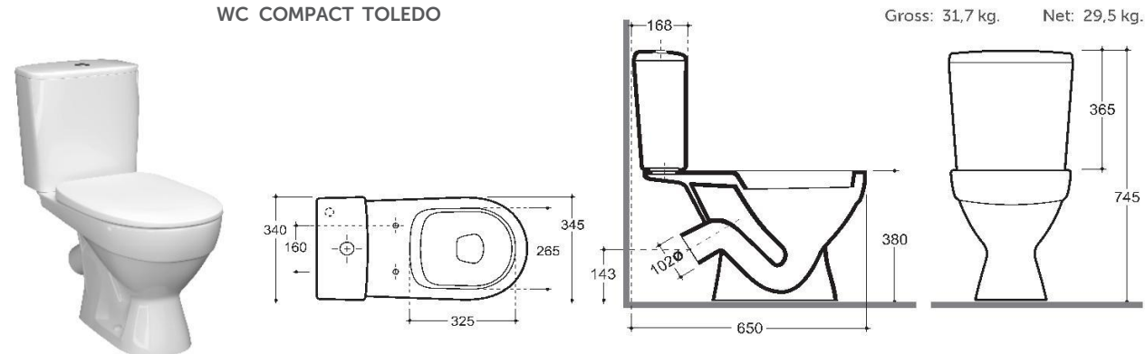
WC COMPACT TOLEDO
