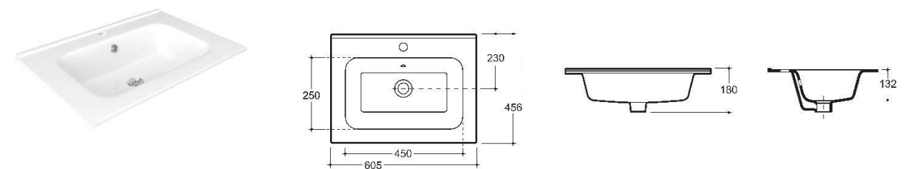
WASH-BASIN GENEVA 60 PLUGGABLE
