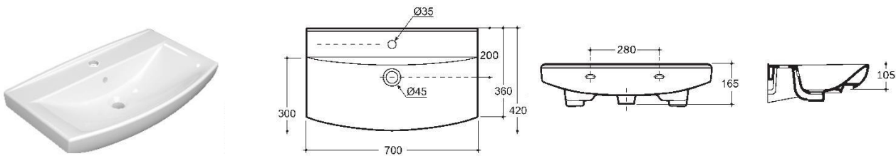
SEMI-RECESSED WASH-BASIN CLAREMONT 70
