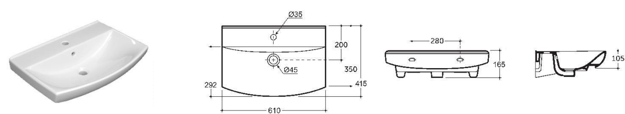
SEMI-RECESSED WASH-BASIN CLAREMONT 60
