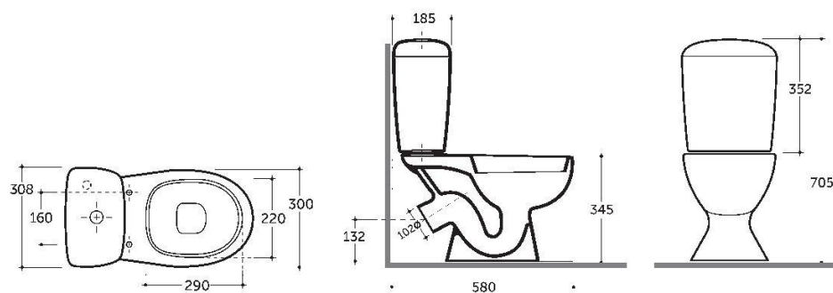
WC COMPACT LITTLE
