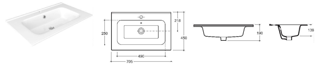
WASH-BASIN GENEVA 70 PLUGGABLE
