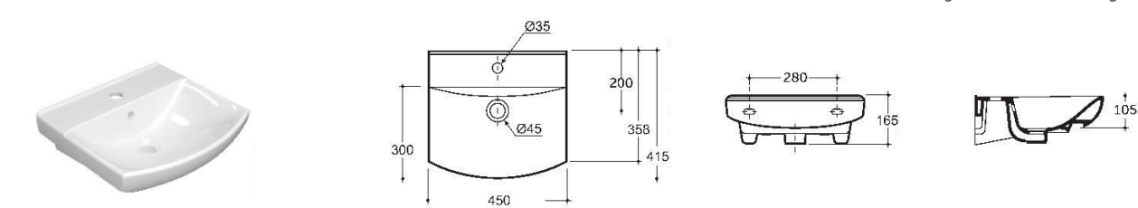
SEMI-RECESSED WASH-BASIN CLAREMONT 45
