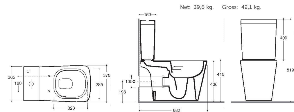
WC COMPACT TOBAGO R
