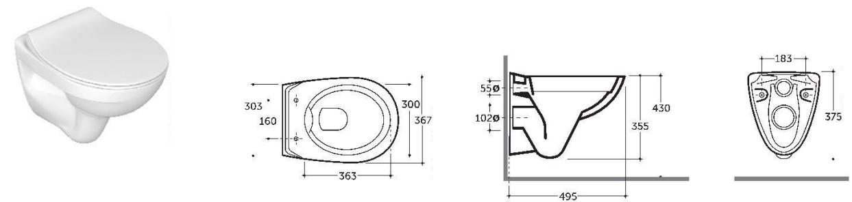
WALL-HUNG WC SANTI R
