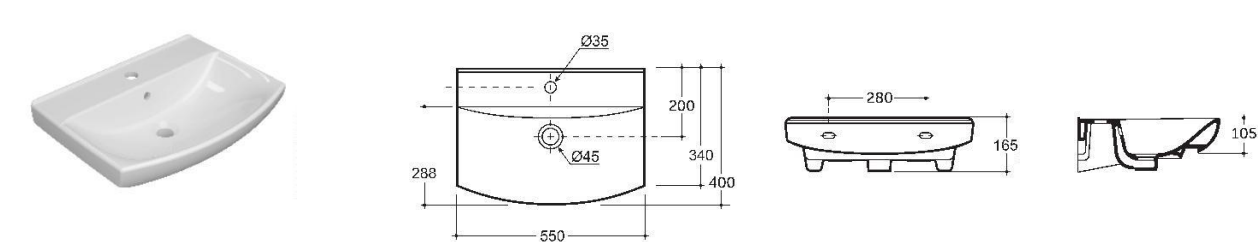
SEMI-RECESSED WASH-BASIN CLAREMONT 55
