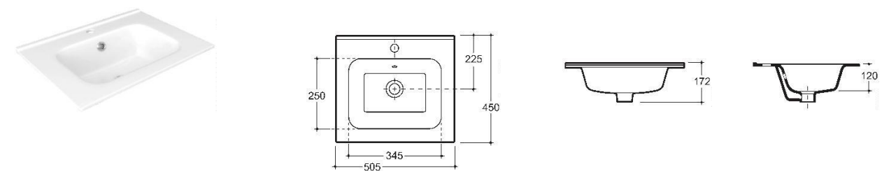
WASH-BASIN GENEVA 50 PLUGGABLE
