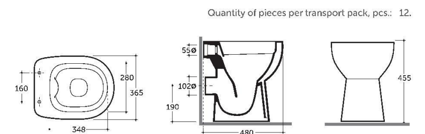
WC ALBANO R OPTIMA PLUS WITHOUT SHELF
