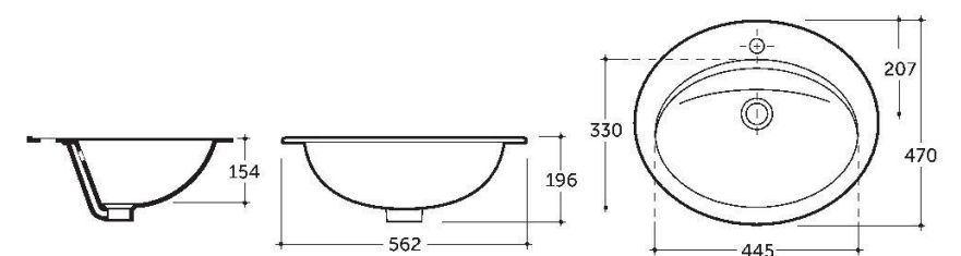
WASH-BASIN TURIN PLUGGABLE
